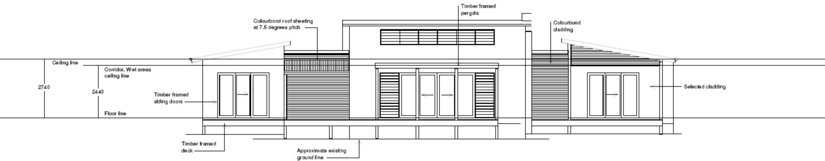
NORTH ELEVATION
