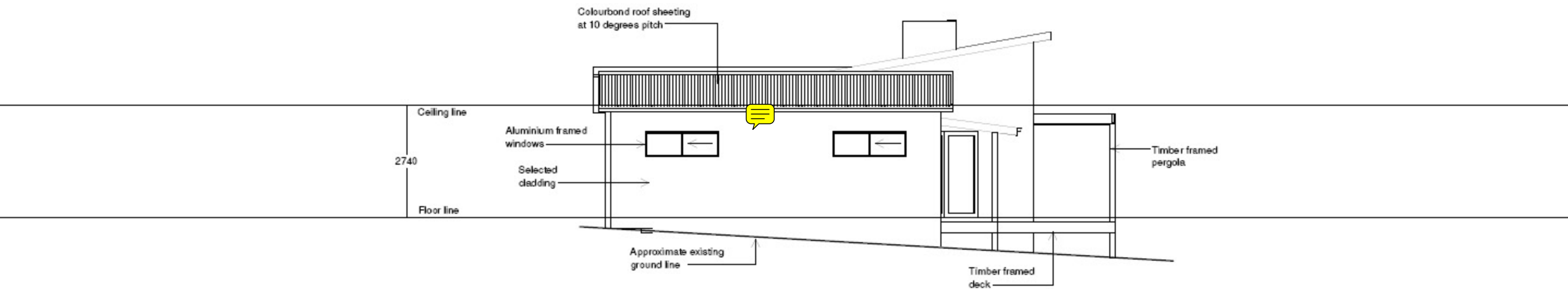
EAST ELEVATION
